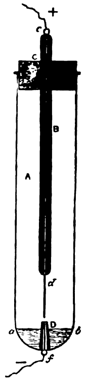
A, Tube into which the liquid to be analysed is poured. B, Capillary tube in which is fixed the platinum wire cd , which forms the upper electrode. C, Cork stopper closing the tube A; it supports B, and permits its being moved with little friction. D, Small capillary tube, slightly conical, covering the lower electrode f . d , Upper electrode. f , Lower electrode. ab , Level of liquid.
